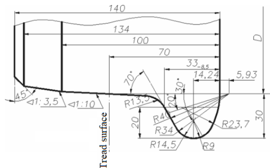
Fig. 4. Dimensions and surface shape of the wheel tread surface
