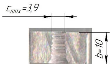
Fig. 3. Photo of a sample cut out of a rail with the dimensions of the wear zone
