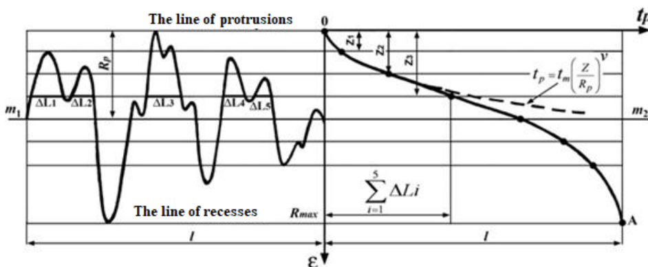
Fig. 2. The material ratio curve (Abbot-Firestone curve): \varepsilon is a profile height; t_p is a supporting length; R_p is the distance from the line of protrusions to the midline (the line m_1 - m_2 ); t_m is the relative supporting length of the profile along the midline (the line m_1 - m_2 ); R_{max} is the distance between the line of protrusions and the line of recesses within the base length of the surface profile l ; Z_j is a row of horizontal levels; \Delta L_i is a width of the protrusions at the level Z_j under consideration
