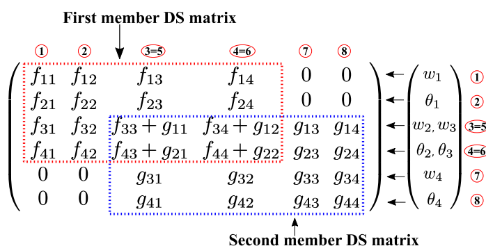
Fig. 4.1.1. The schematic representation of the global DS assembly process for the case of a two-span beam. Dashed rectangles show the member DS matrices. The overlap between two rectangles defines common degrees of freedom of both members. The overlap between matrices ensures that conditions of continuity of the structure are preserved. The corresponding degrees of freedom are numbered
